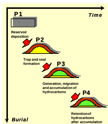
Fig. 3.1 Geochronological risk assessment
