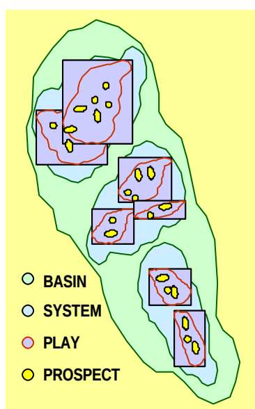
Fig. 5.2 Schematic illustration of the relation between basin, petroleum system, play and prospect
