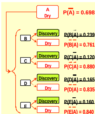
Fig. 4.6 Conditional probabilities in B, C, D and E, given that A is dry.
