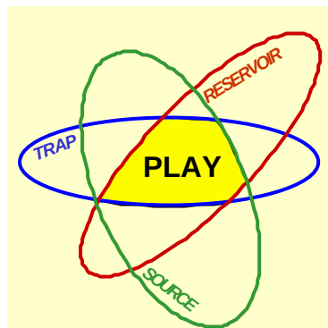
Figure 5.1 Schematic illustration of play definition
