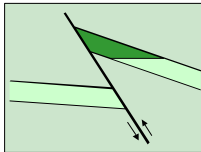
G. Fault block (reverse)
