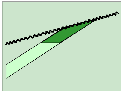
E. Trap formed by truncation
