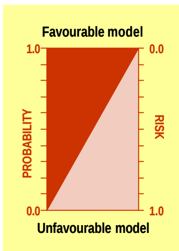
Fig. 3.8 Schematic relation between favourable and unfavourable models.
