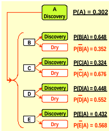
Fig. 4.5 Conditional probabilities in B, C, D and E, given a discovery in A.
