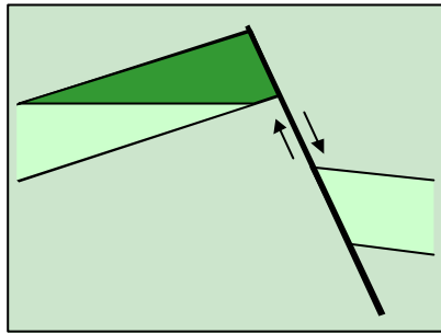
C. Rotated fault block (normal)
