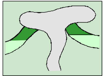
D. Traps formed by salt diapirism
