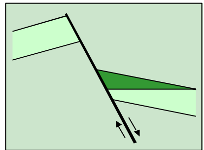
F. Downthrown fault block
