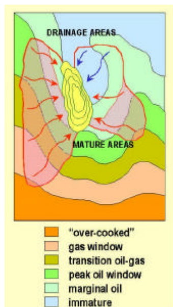
Fig. 3.15 Example of a maturity map with drainage areas and migration paths.
