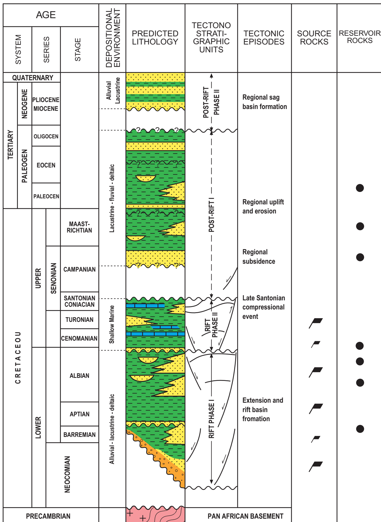
Logone Birni Basin - Predicted Lithology, Tectono-stratigraphic Development, Source and Reservoir Rocks
